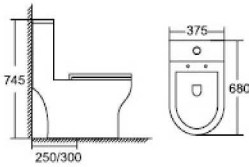
SV2081 One-Piece Toilet Flushing System: Washdown Size: 680x375x745mm P-trap: 180mm S-trap: 250/300mm
