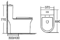
SV2027 One-Piece Toilet Flushing System: Tomado Size: 690x370x770mm S-trap: 300/400mm
