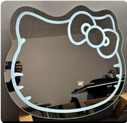
SVBM002 Dimension: 24*36" (610*914mm) or customized Mirror: 3/4/5mm Copper Free Silver Mirror Switch: Touch/motion sensor/or no switch Light source: LED SMD 2835, 120 or 60pcs/m Color Temperature: 3000K, 4000K, 6000K ICRI: > 90 Voltage: AC 110~240V, 50/60Hz
