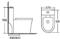
SV2073 One-Piece Toilet Flushing System: 2 Super Siphonic Size: 680x370x765mm S-trap: 300/400mm
