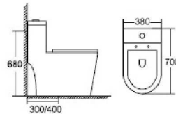
SV2076 One-Piece Toilet Flushing System: 2 Super Siphonic Size: 700x380x680mm S-trap: 300/400mm
