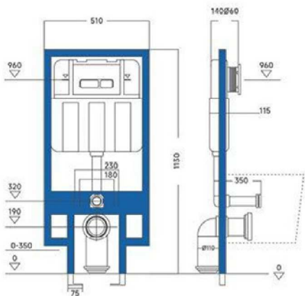
SVT280 Concealed-water tank
