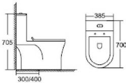
SV2084 One-Piece Toilet Flushing System: 4 Super Siphonic Size: 700x385x705mm S-trap: 300/400mm
