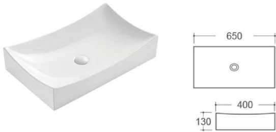
SV8420 Art Basin Size: 650x400x130mm Above Counter Mounted
