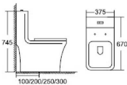
SV2012 One-Piece Toilet Flushing System: Siphonic Size: 670x375x745mm S-trap: 100/200/250/300mm
