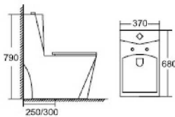
SV2011 One-Piece Toilet Flushing System: Siphonic Washdown Size: 680x370x790mm P-trap: 180mm S-trap: 250/300mm
