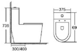
SV2080 One-Piece Toilet Flushing System: 2 Super Siphonic Size: 690x375x735mm S-trap: 300/400mm
