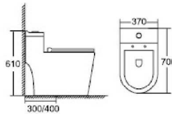
SV2083 One-Piece Toilet Flushing System: Siphonic Size: 700x370x610mm S-trap: 300/400mm
