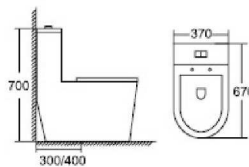
SV2077 One-Piece Toilet Flushing System: 2 Super Siphonic Size: 670x370x700mm S-trap: 300/400mm
