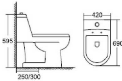
SV2019 One-Piece Toilet Flushing System: Siphonic Size: 690x420x595mm S-trap: 250/300mm
