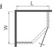
SVJZR309 / Pivot 2 fixed 1 outward/inward
