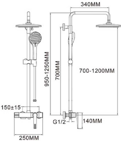
SVD01004HJ BRASS/BLACK&ROSE GOLD
