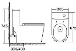
SV2078 One-Piece Toilet Flushing System: 1 Super Siphonic Size: 675x385x745mm S-trap: 300/400mm
