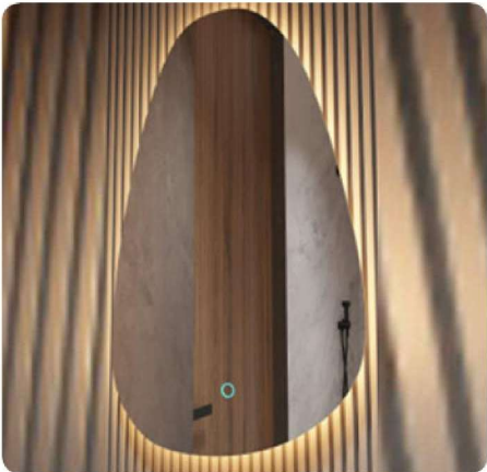
SVBM001 Dimension: 24*36" (610*914mm) or customized Mirror: 3/4/5mm Copper Free Silver Mirror Switch: Touch/motion sensor/or no switch Light source: LED SMD 2835, 120 or 60pcs/m Color Temperature: 3000K, 4000K, 6000K ICRI: > 90 Voltage: AC 110~240V, 50/60Hz
