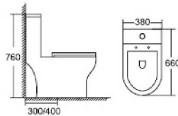
SV2075 One-Piece Toilet Flushing System: Washdown Size: 660x380x760mm P-trap: 180mm S-trap: 300/400mm
