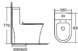
SV2074 One-Piece Toilet Flushing System: 2 Super Siphonic Size: 690x380x770mm S-trap: 300/400mm
