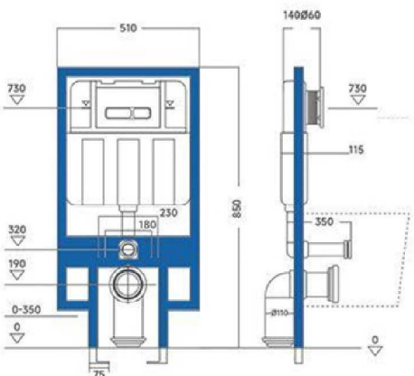
SVT280-85 Concealed-water tank
