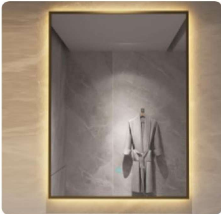
SVBM045 Dimension: 24*36" (610*914mm) or customized Mirror: 3/4/5mm Copper Free Silver Mirror Switch: Touch/motion sensor/or no switch Light source: LED SMD 2835, 120 or 60pcs/m Color Temperature: 3000K, 4000K, 6000K ICRI: > 90 Voltage: AC 110~240V, 50/60Hz
